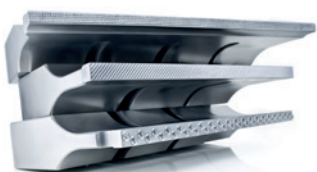
Welding sonotrodes with different structures
