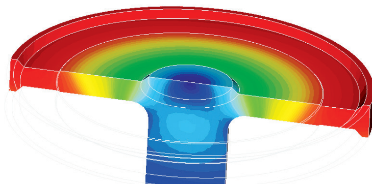
FEM view of a roll seam sonotrode mounted on one side
